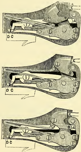
Scott's Automatic Intercepting Safety Bolt.
